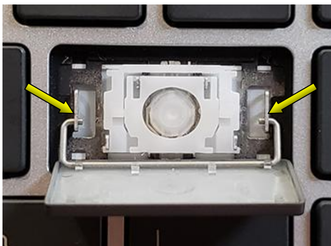
Insert stabilizer bar(s) into the appropriate brackets
